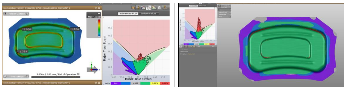
Figure 11 – Optimization objective to simultaneously match nominal draw in remove splitting for two new processing parameter test sets from left) GM and right) Ford.
